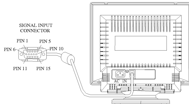
Figure 2 Connecting Cables
