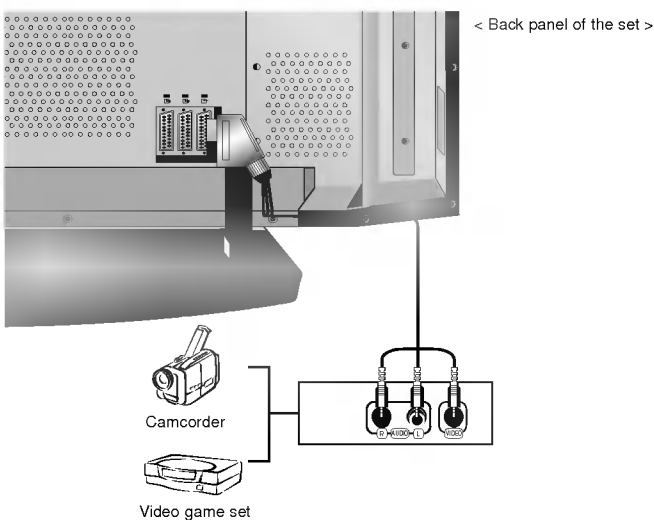
< Back panel of the set >
