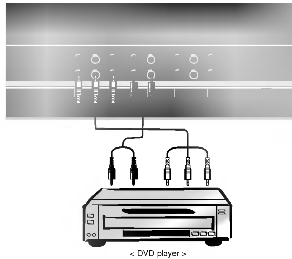
< Back panel of the set >
