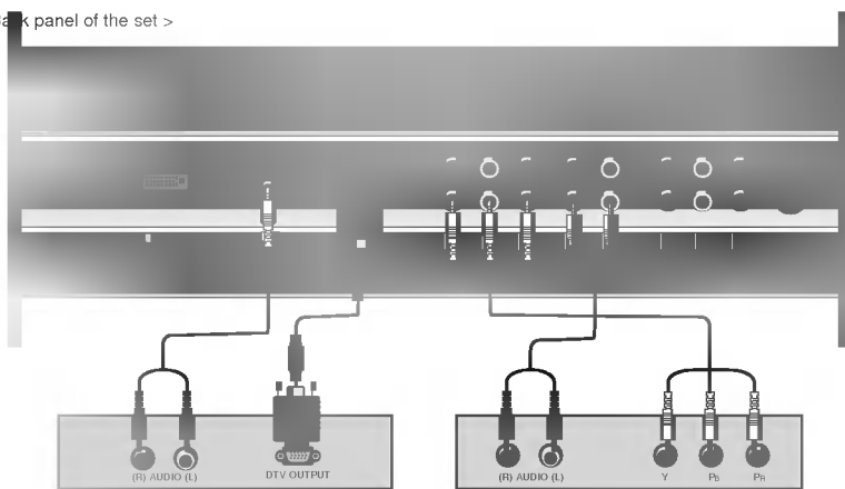
< Digital Set-top box >
