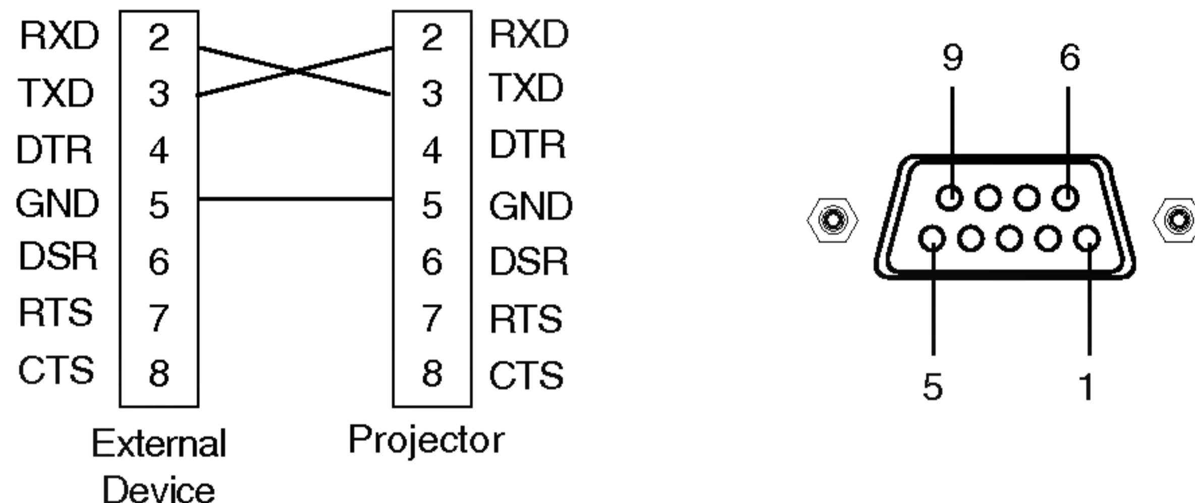
<Fig.1, RS-232 Interface Cable>
