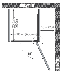
Built-In Installation
