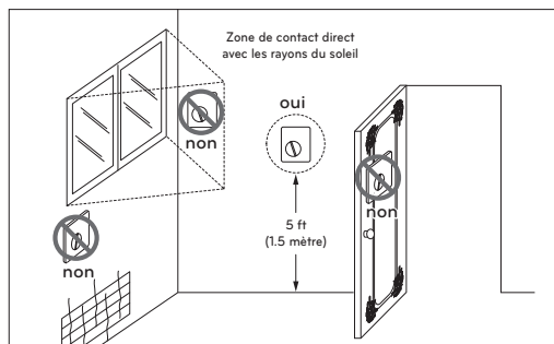
Thermostat
