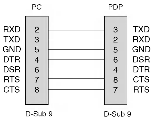
7-Wire Configurations (Standard RS-232C cable)
