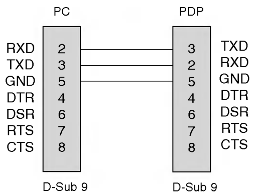
3-Wire Configurations (Not standard)
