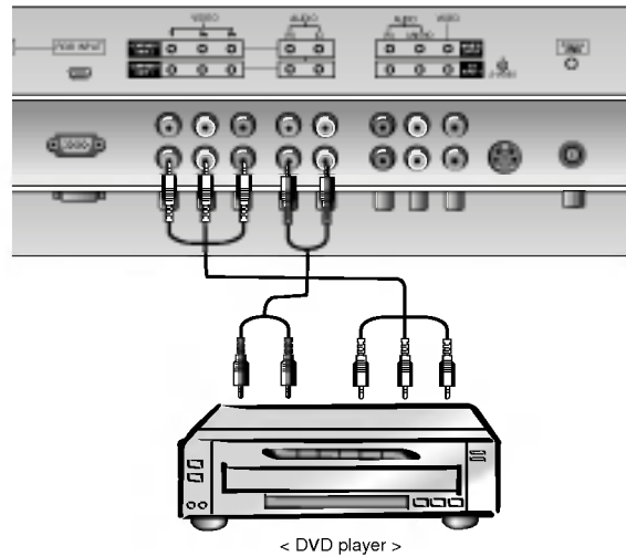
< DVD player >
