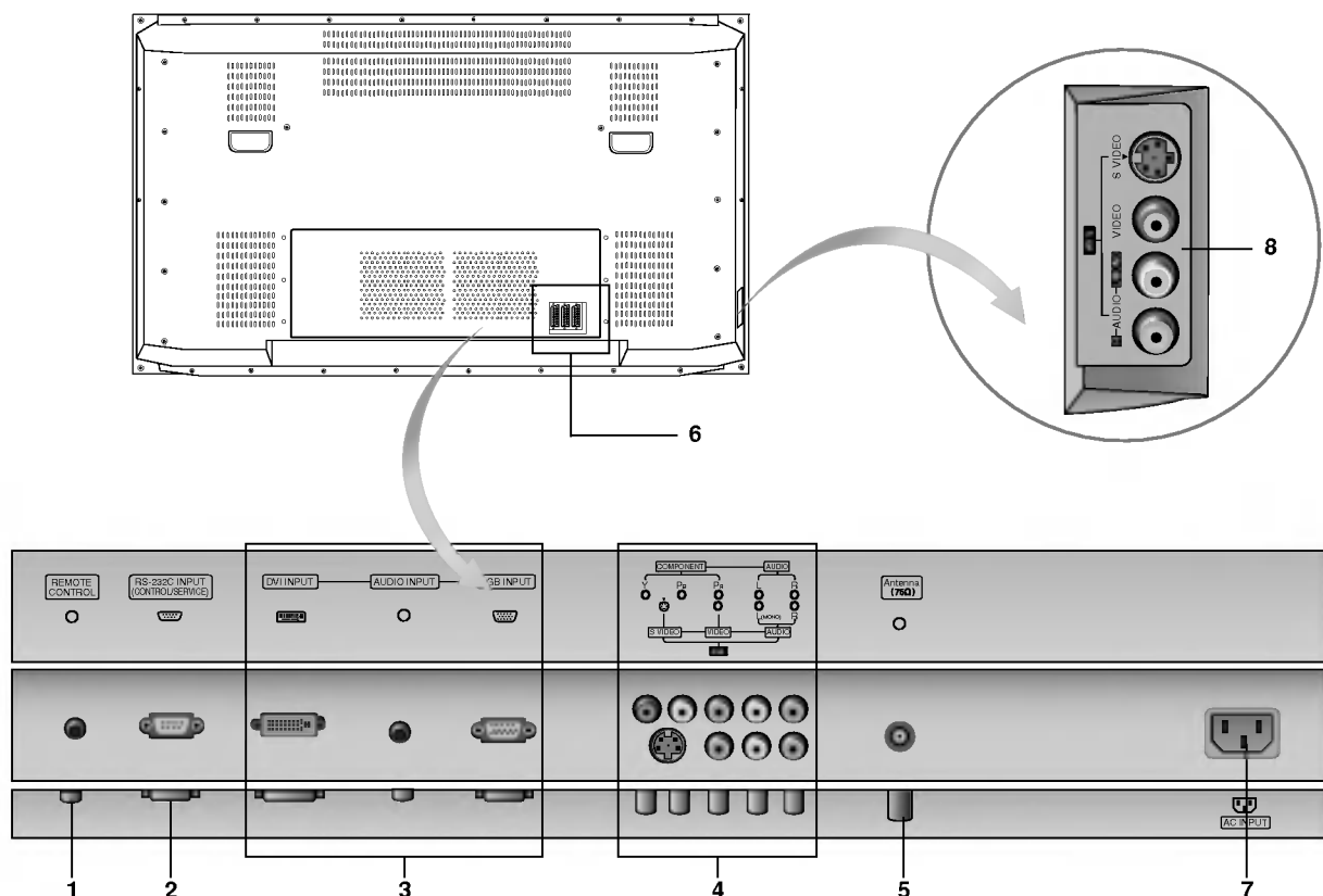
<Back Panel>
