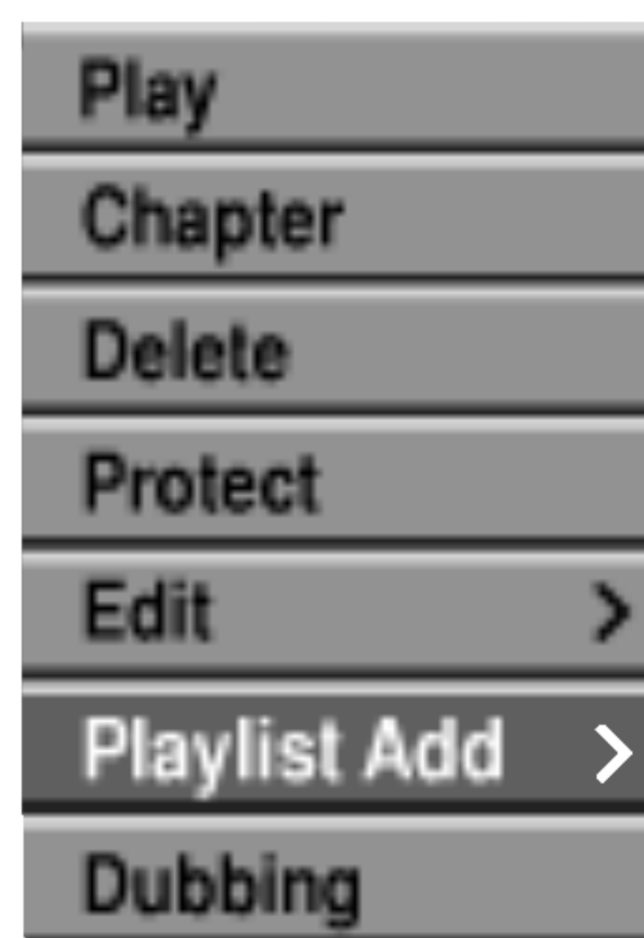
Title List-Original
