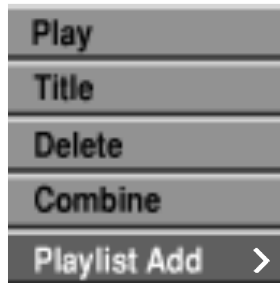
Chapter List-Original
