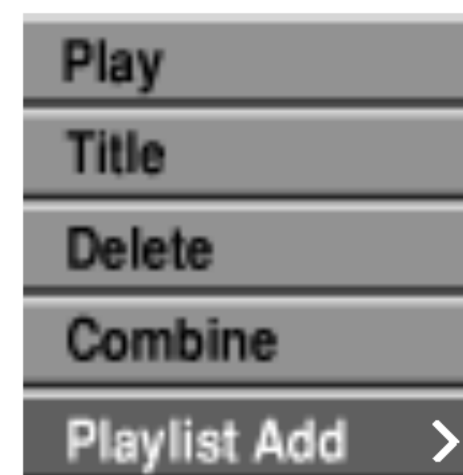
Chapter List-Original
