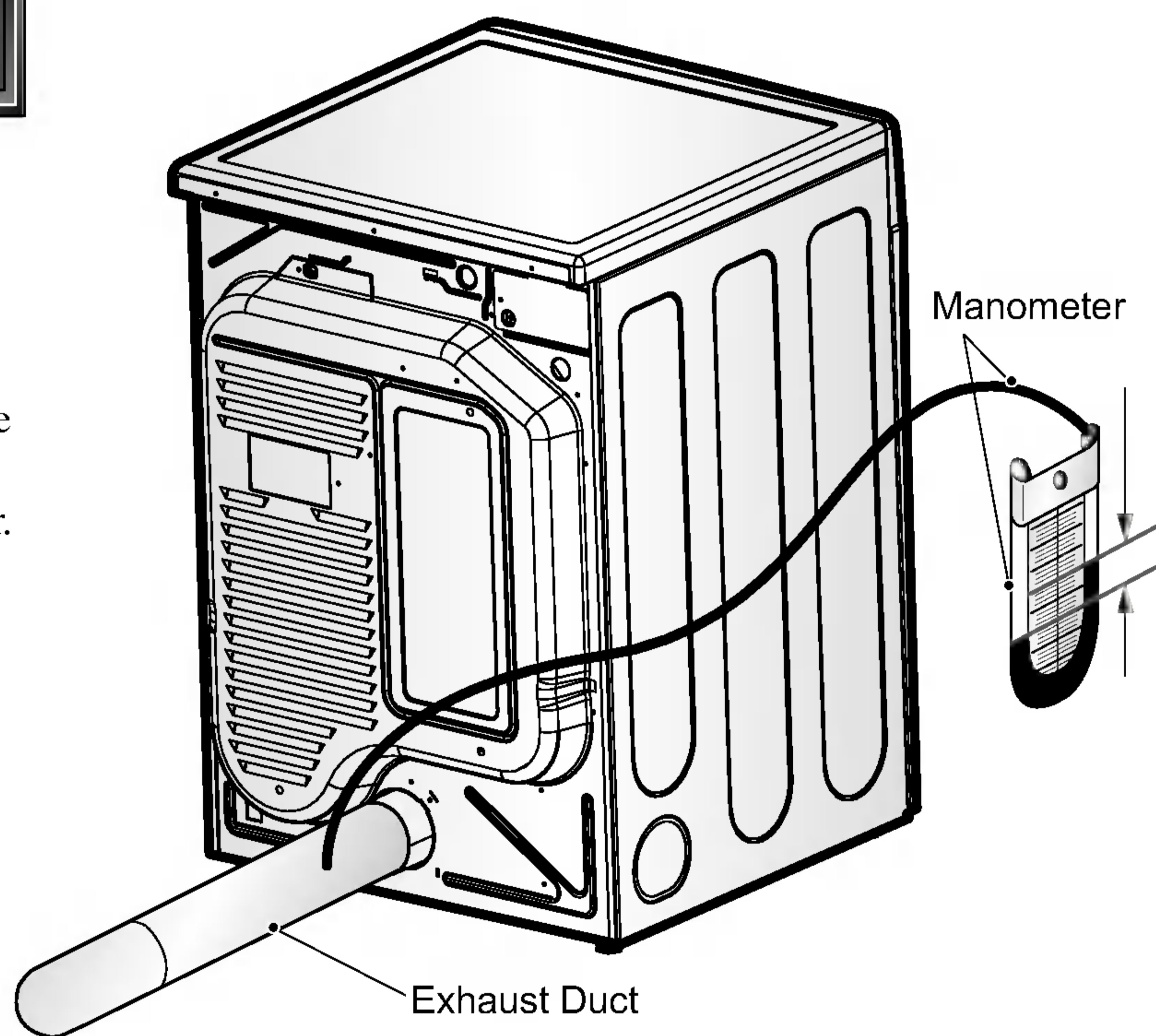
Measuring Static pressure
