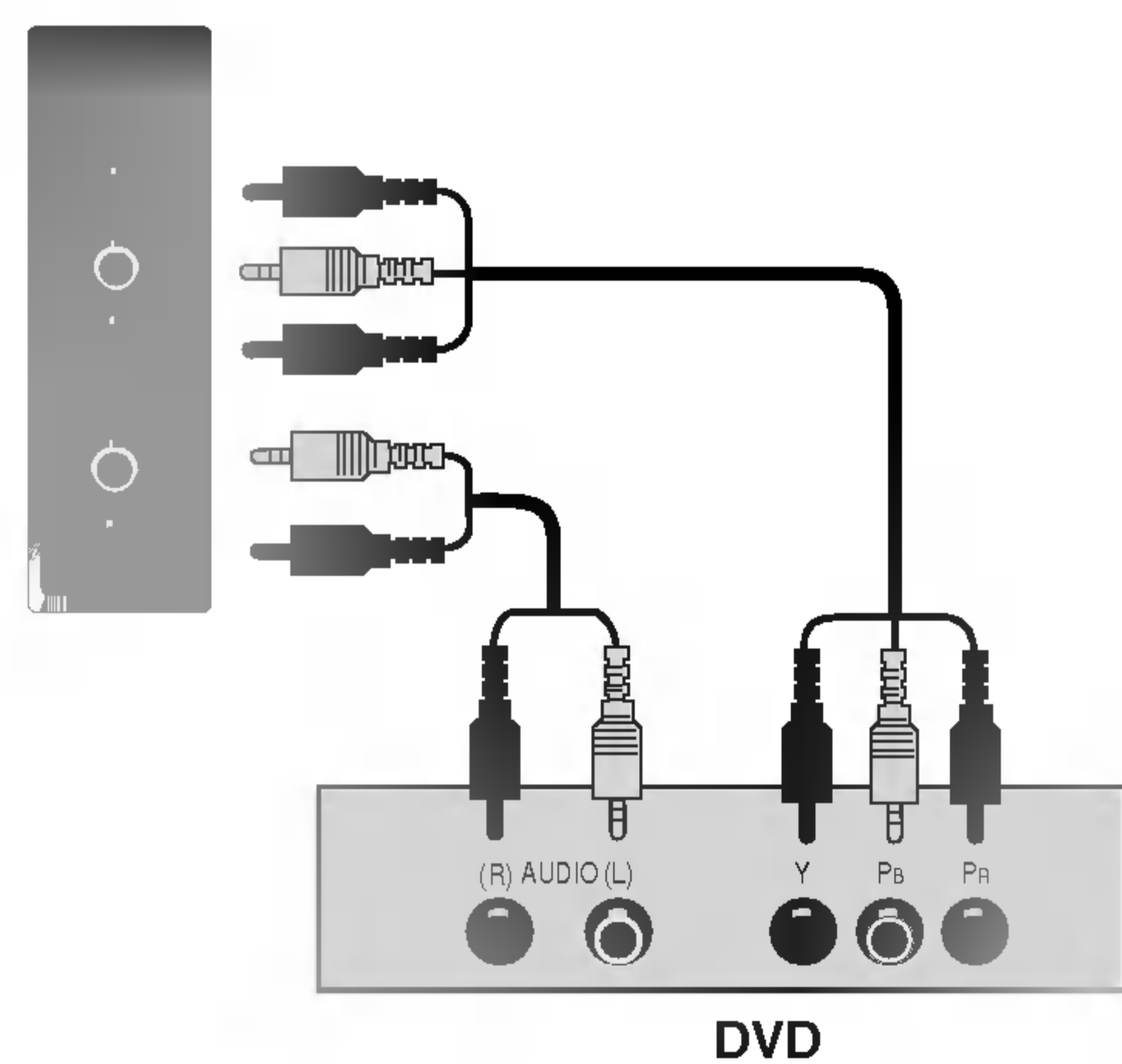
Side Panel
