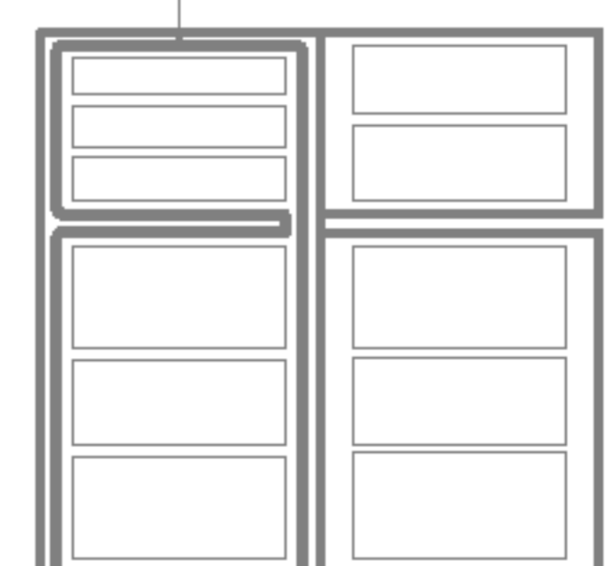
Anti-Condensation Pipe
