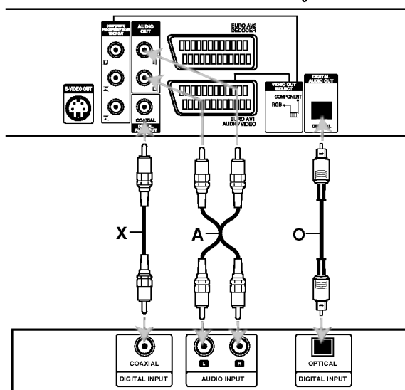
Pojačalo (Receiver)
