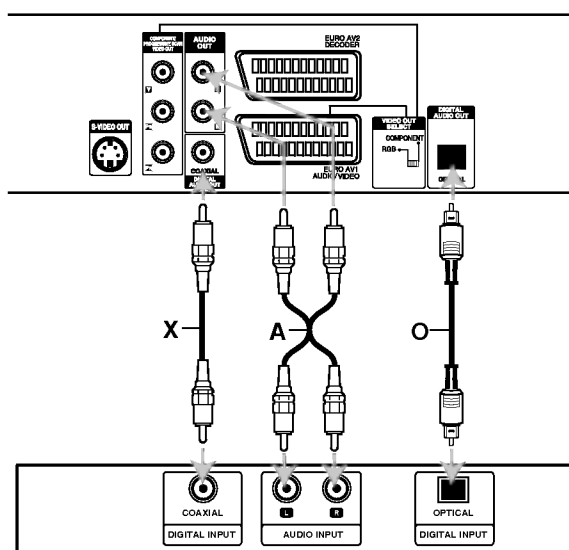
Amplificator (Receiver)
