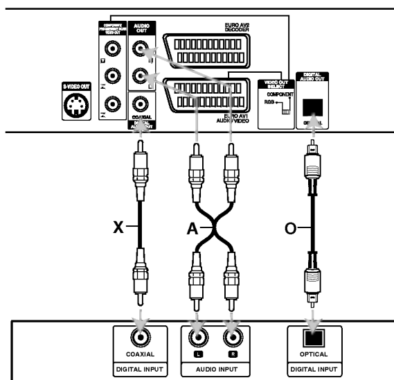
Versterker (Ontvanger)
