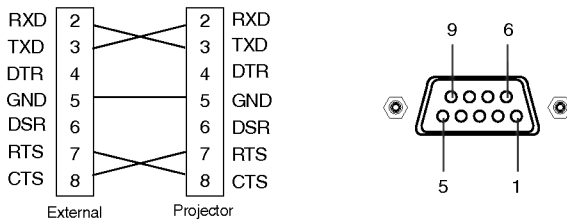
<Fig.1, RS-232 Interface Cable>
