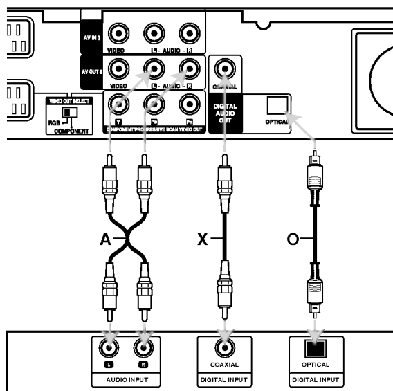
Pojačalo (Receiver)
