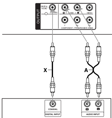
Amplifier (Receiver)
