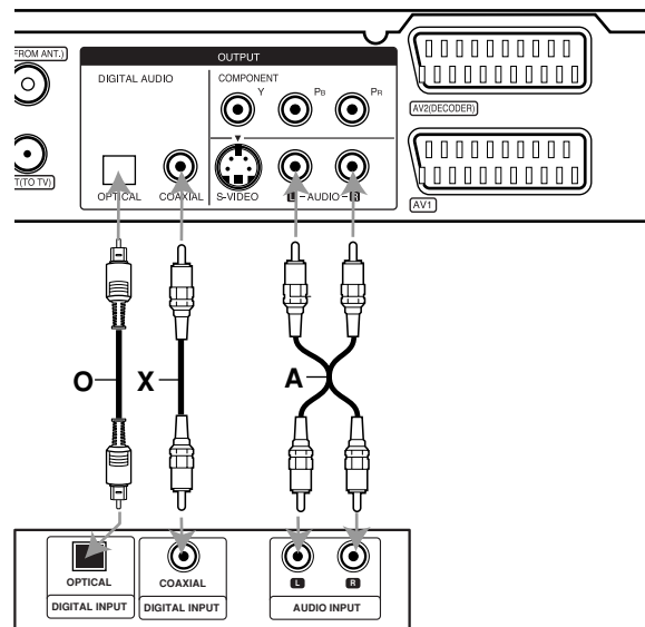
Pojačalo (Receiver)
