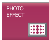
PHOTO EFFECT (EFFECT FOTO)
