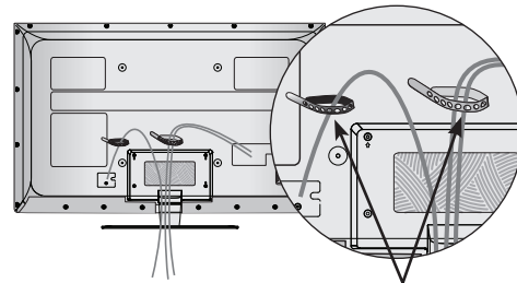
Cable Holder
