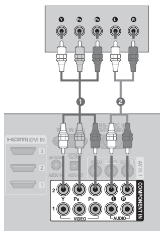
Y, Cb/Pb, Cr/Pr
