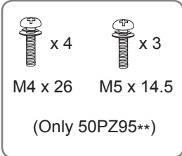
Screw for assembly
