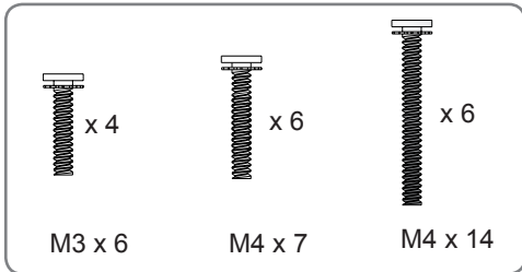
Bolts for stand and wall mounting bracket assembly
