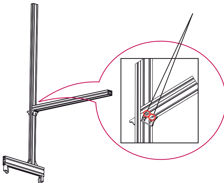
Example of Assembled Stand
