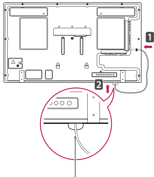
IR Receiver cable
