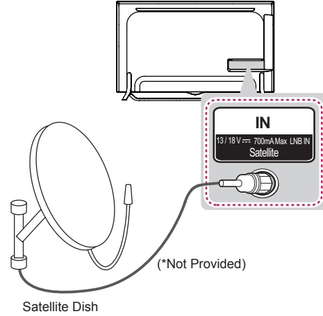
Satellite Dish
