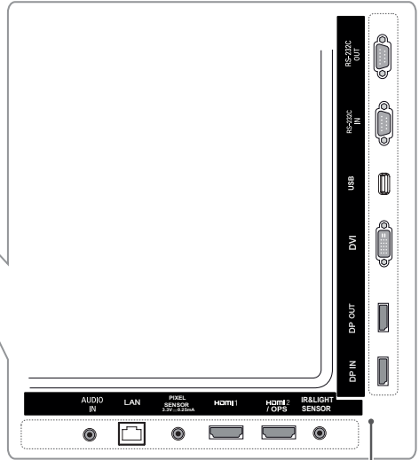
Tilkoblingspanel
