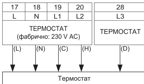
За Hydrosplit 1-Pipe
