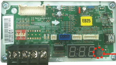
TACT-SW1
