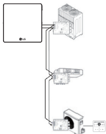
<Correct example : RS485 BUS format connection>
