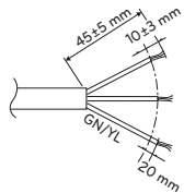
<Sheath removal guide>
