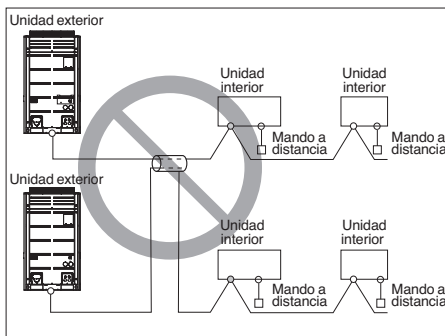
Cable multi-capas
