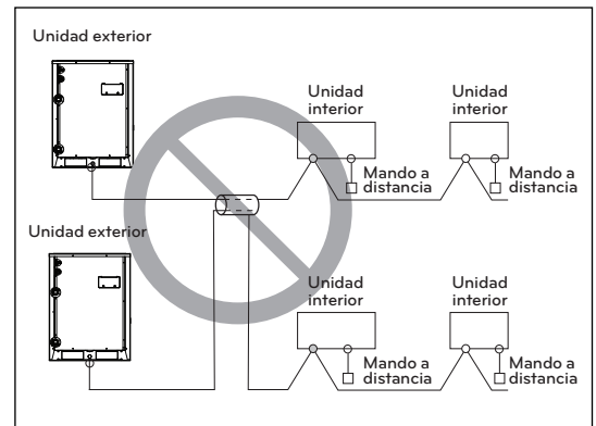
Cable multi-capas
