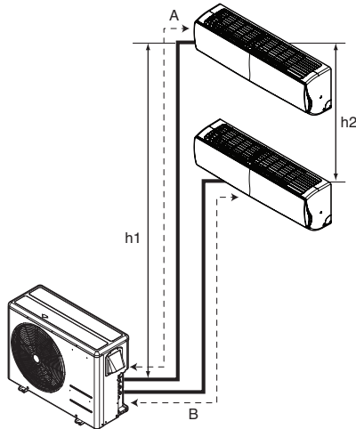
Type multituyaux
