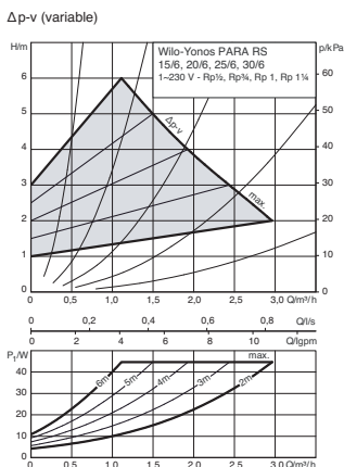
Tolerances of each curve according to EN 1151-1:2006
