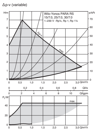
Tolerances of each curve according to EN 1151-1:2006
