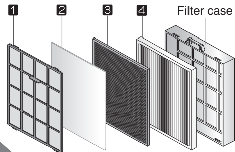
Filter system (Only the filter section is described.)
