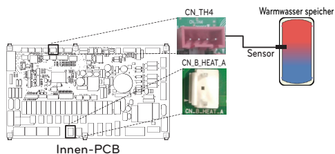
Innen-PCB
