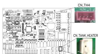
Innen-PCB
