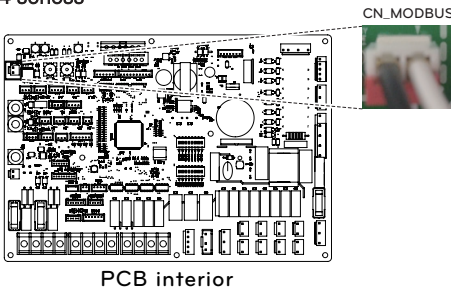
PCB interior
