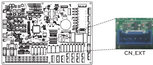
PCB interior
