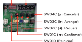
DIP-SW01 7-Segmentos
