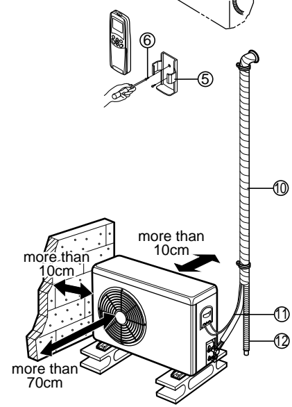
(Floor Mounting)
