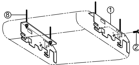
(Ceiling/Wall Mounting)
