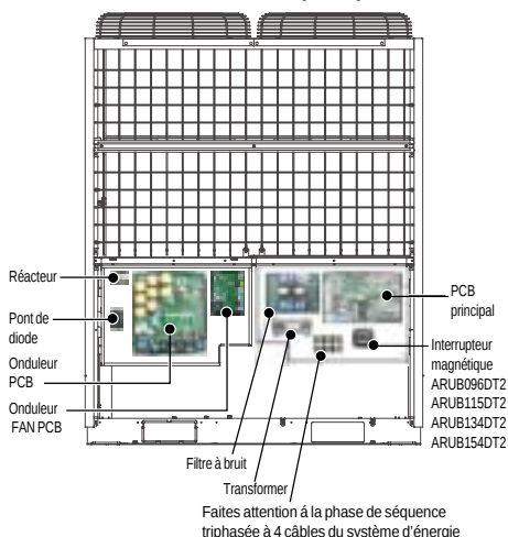
CHASSIS UW1(460V)
