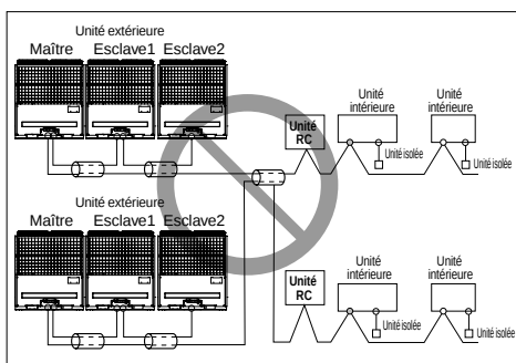
Câble multi-brins
