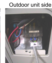
Main wiring (Plug / MCB area)
