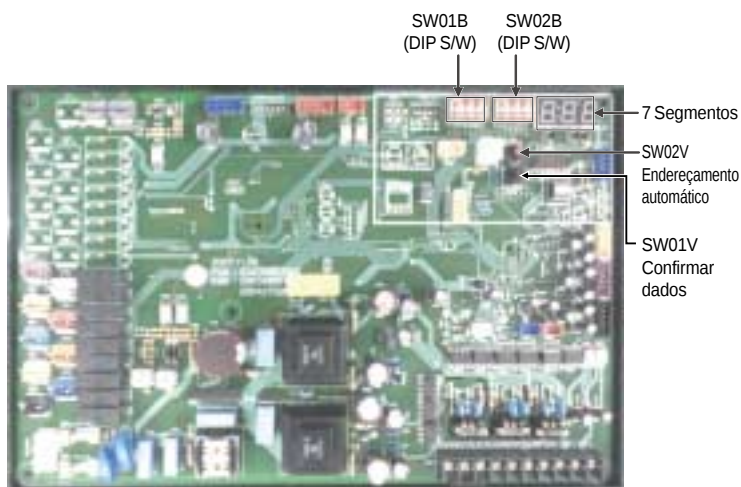
PCB Principal
