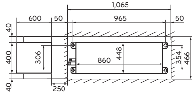
TU Chassis
