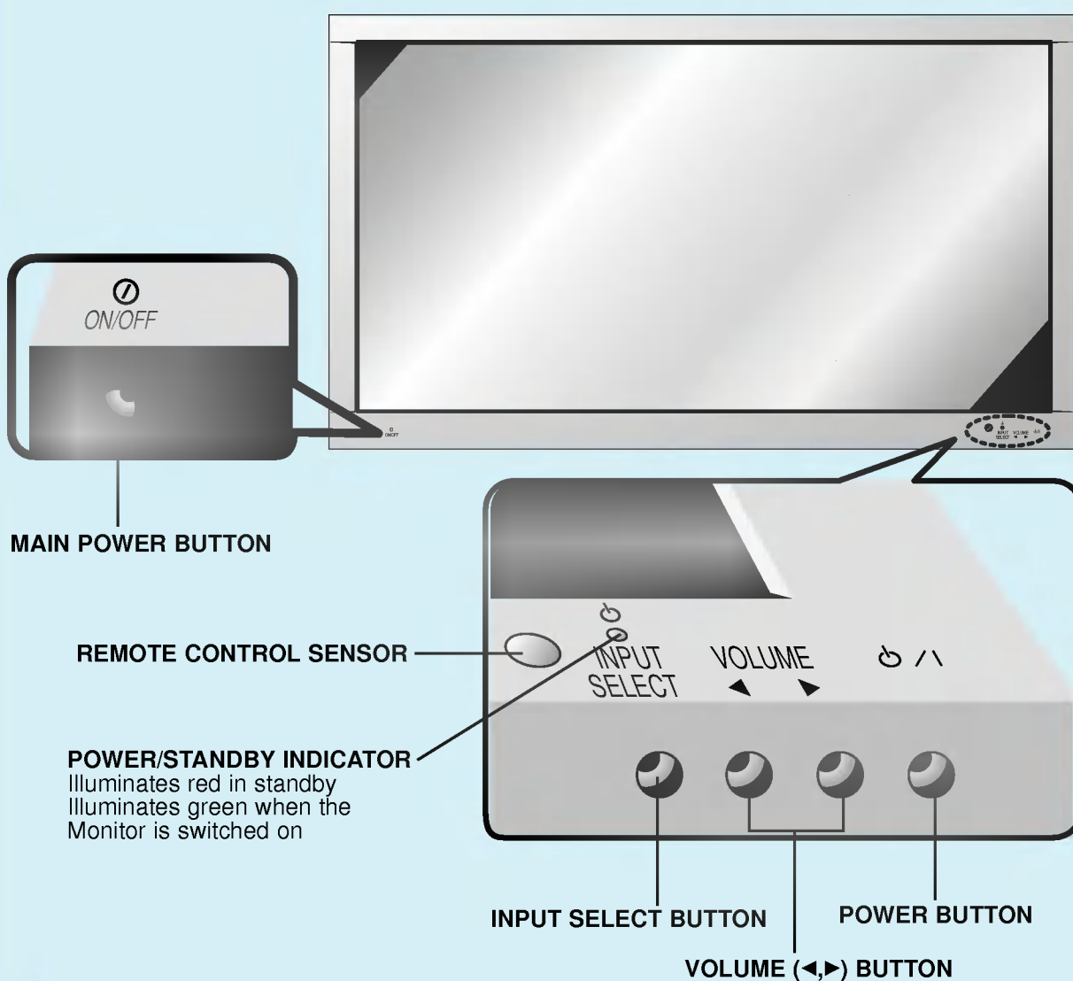
<Front Panel>
