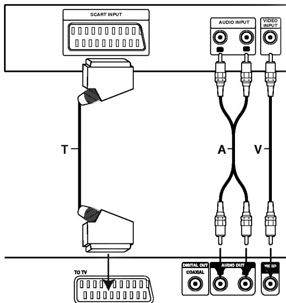
Painel traseiro do televisor
