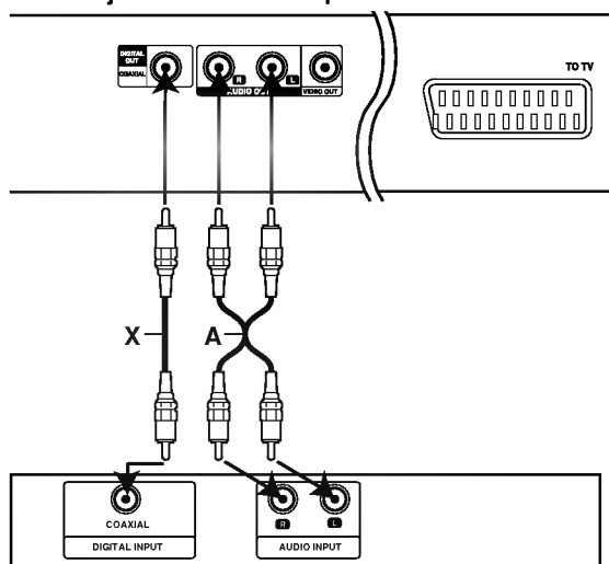
Versterker (Ontvanger)
