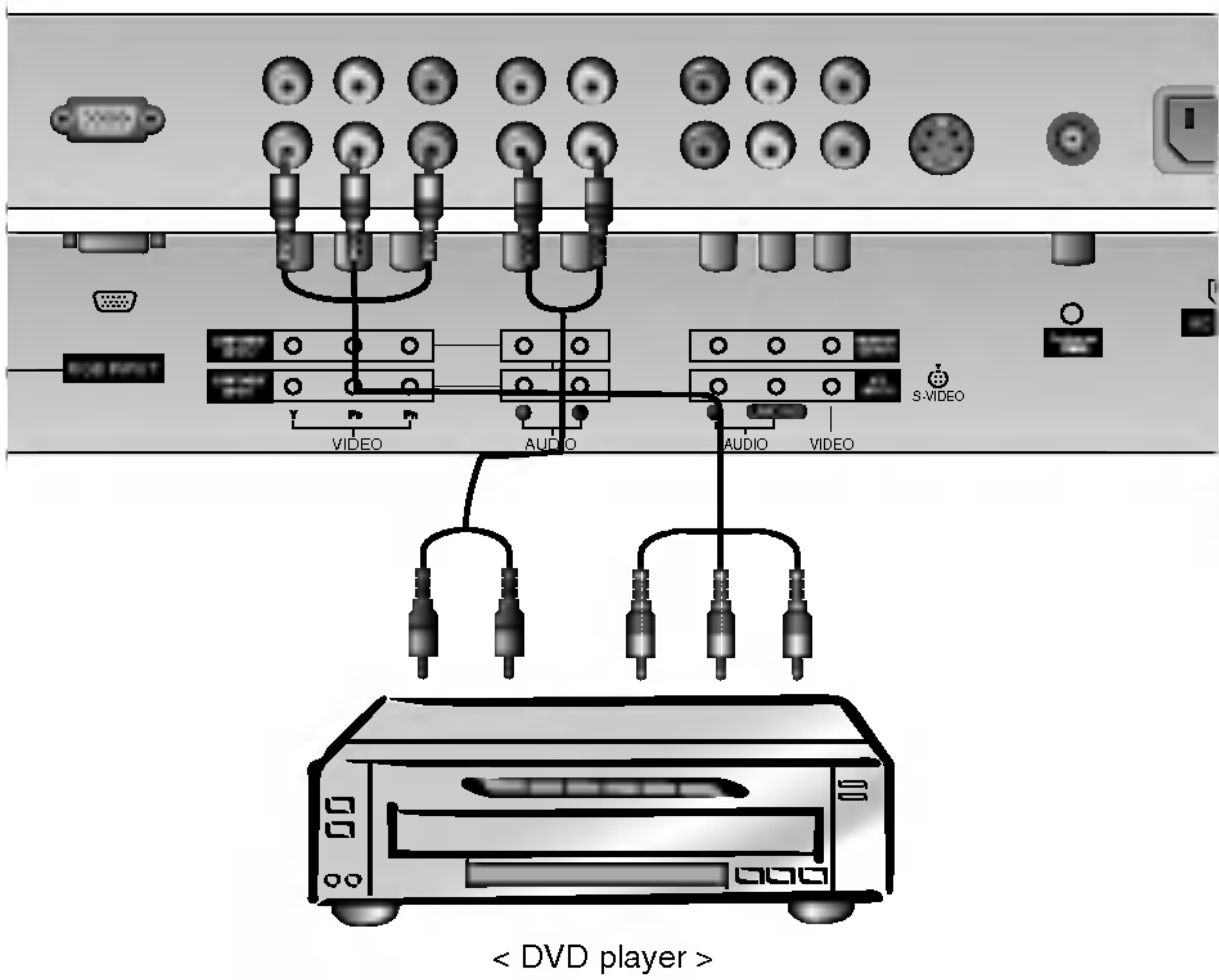
< Back panel of the set >
