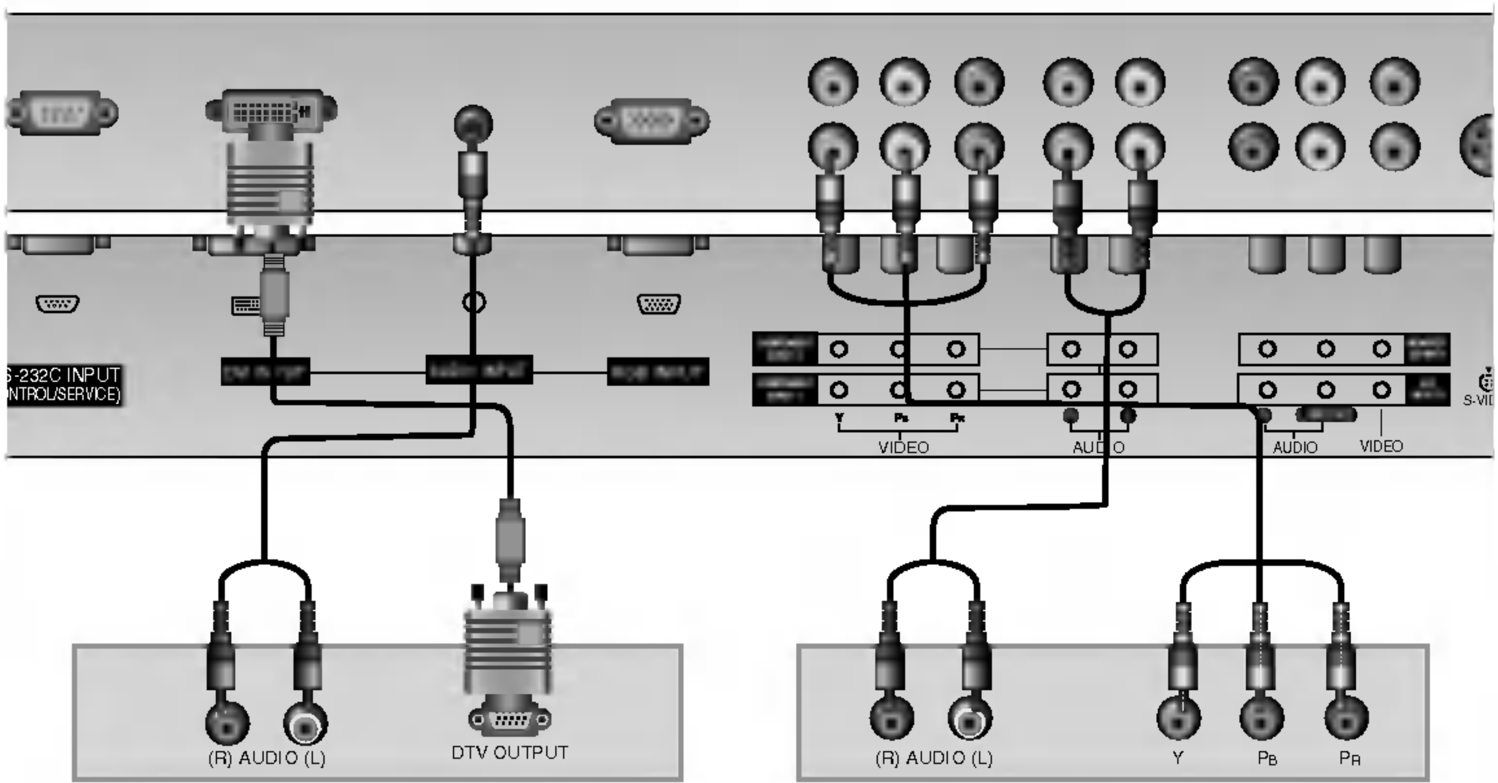
< Back panel of the set >
