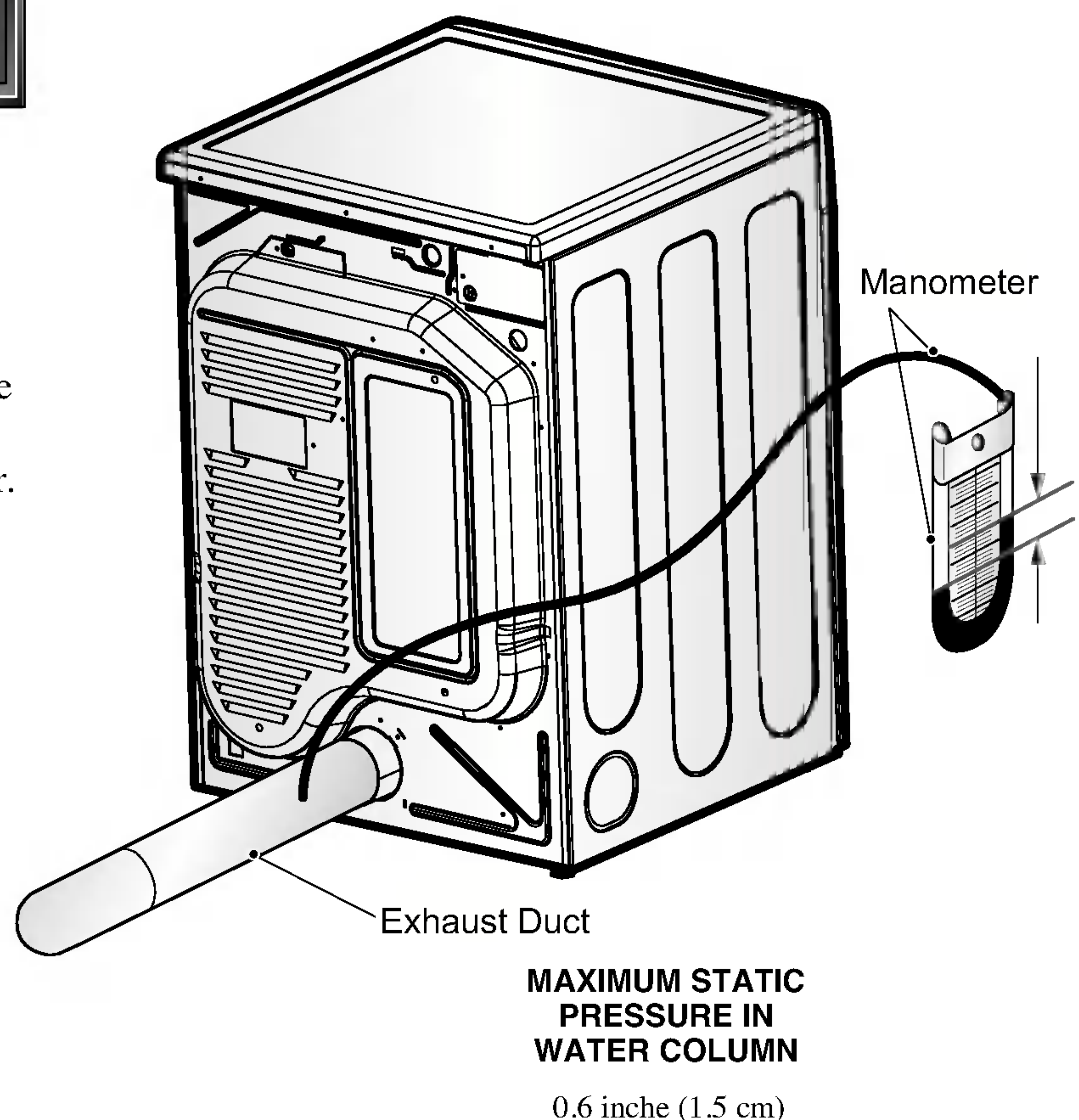
Measuring Static pressure
